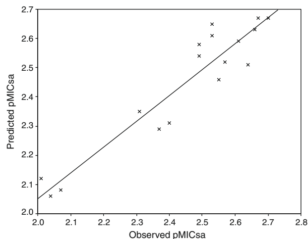
Figure 1. Plot of predicted pMICsa values against the experimental pMICsa values for the linear regression developed model by Eq. (1).
